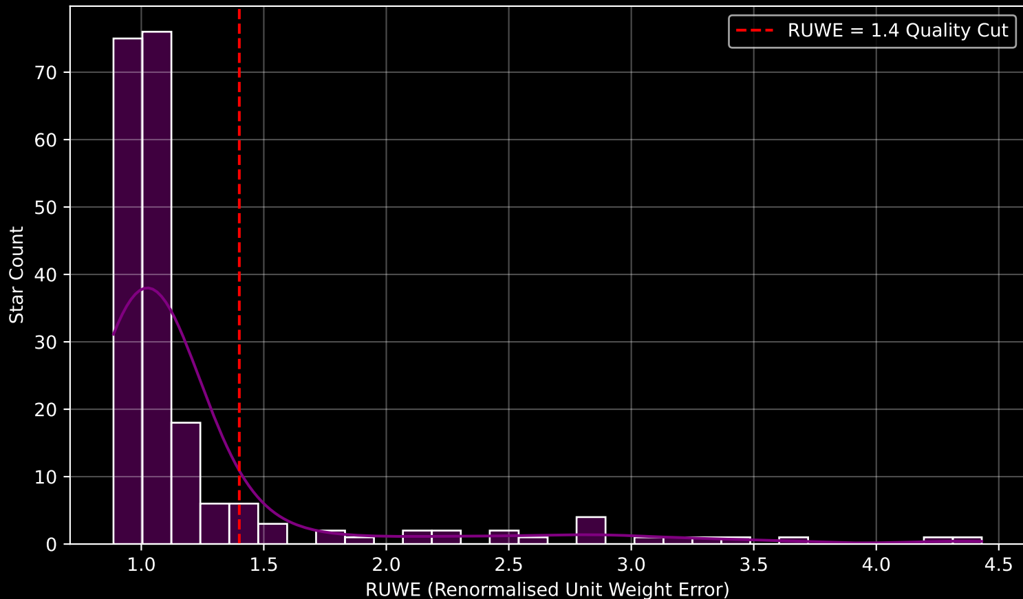
GAPOGEE DR17 Field [K2_C5_210+25_btx] RUWE Distribution (n= 205)
