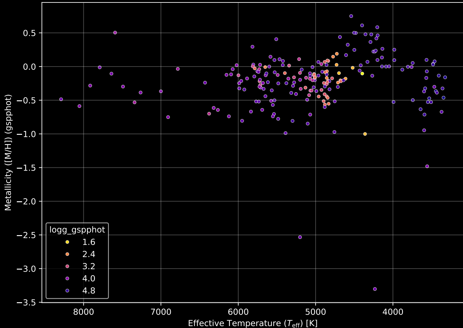
APOGEE DR17 Field: [K2_C5_210+25_btx] Stellar Population Parameters (n= 211)
