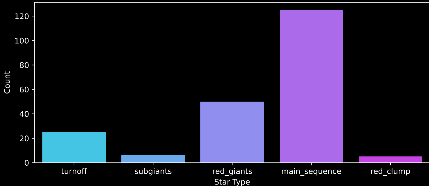
APOGEE DR17 Field: [K2_C5_210+25_btx] Count plot of Star Type
