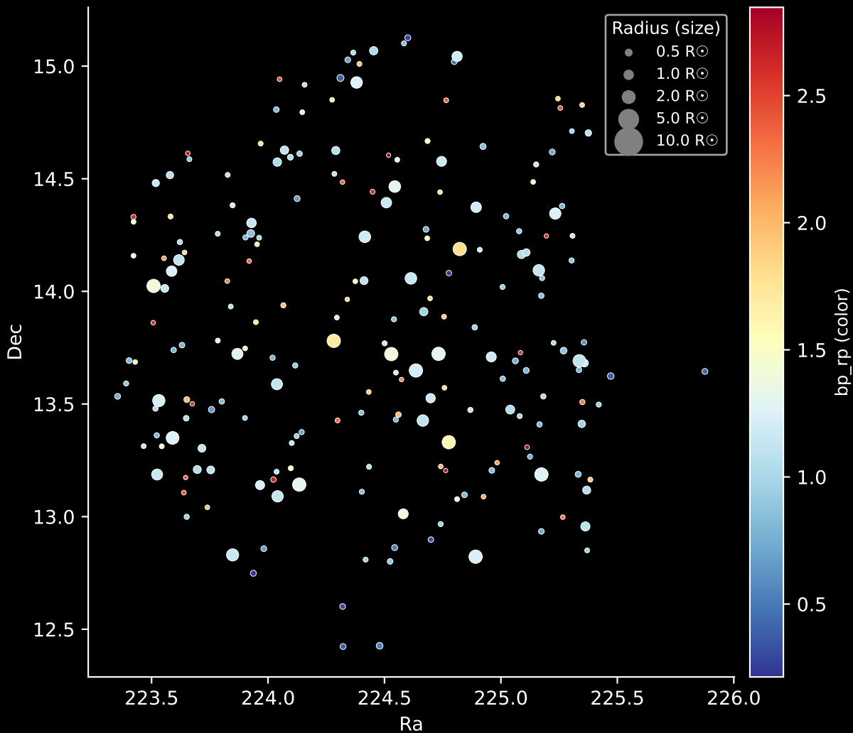
APOGEE DR17 Field: [K2_C5_210+25_btx] Stars: 211
