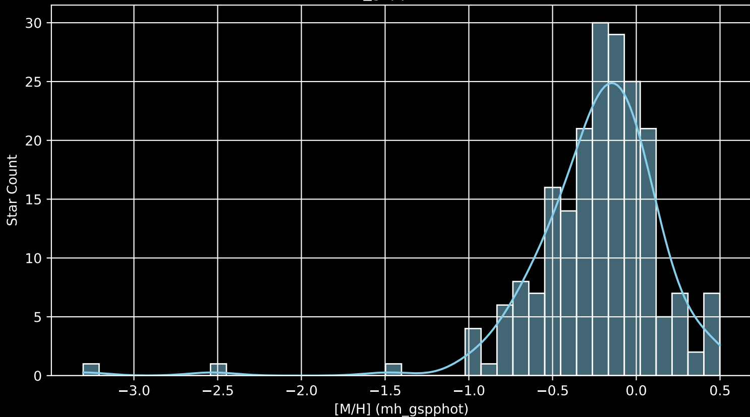
APOGEE DR17 Field: [K2_C5_210+25_btx [M/H] (mh_gspphot) (n= 206)
