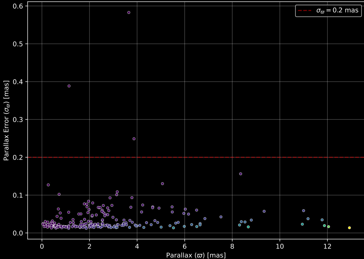
APOGEE DR17 Field: [K2_C5_210+25_btx] Parallax Quality (n= 211)
