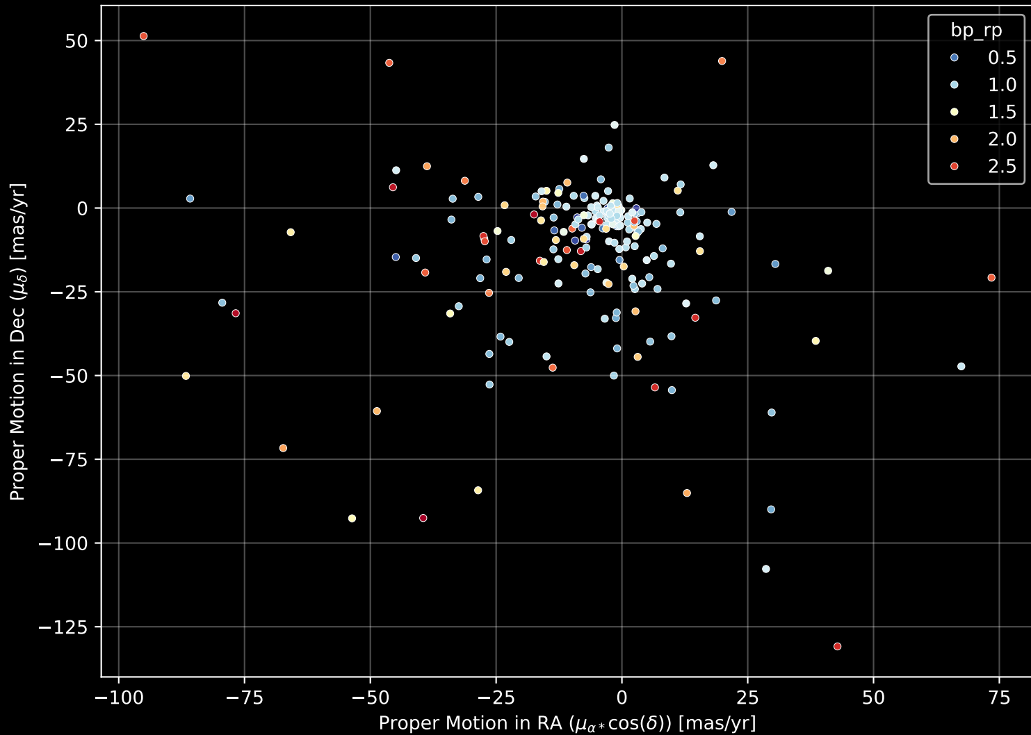
APOGEE DR17 Field: [K2_C5_210+25_btx] Proper Motion Diagram (n= 211)
